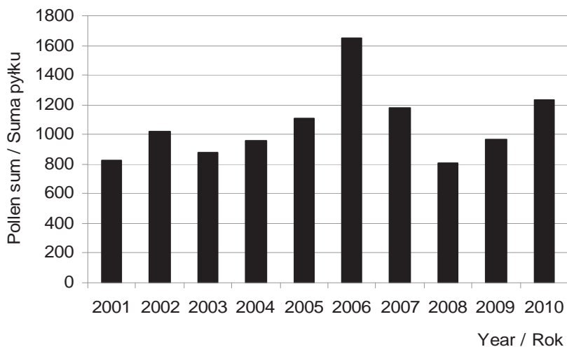
Fig. 4. Comparison annual total sums of Corylus pollen grains in 2001–2010
