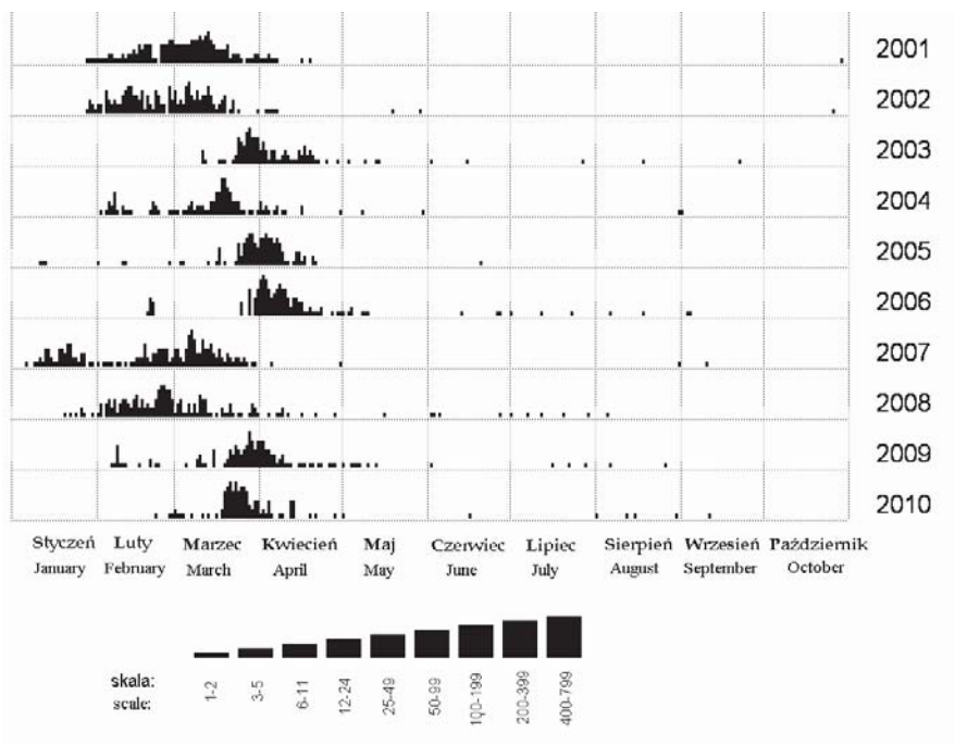
Fig. 2. The airborne Corylus pollen calendar for Lublin in 2001–2010
