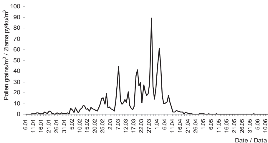
Fig. 3. The hazel pollen season pattern (means for 2001–2010)
