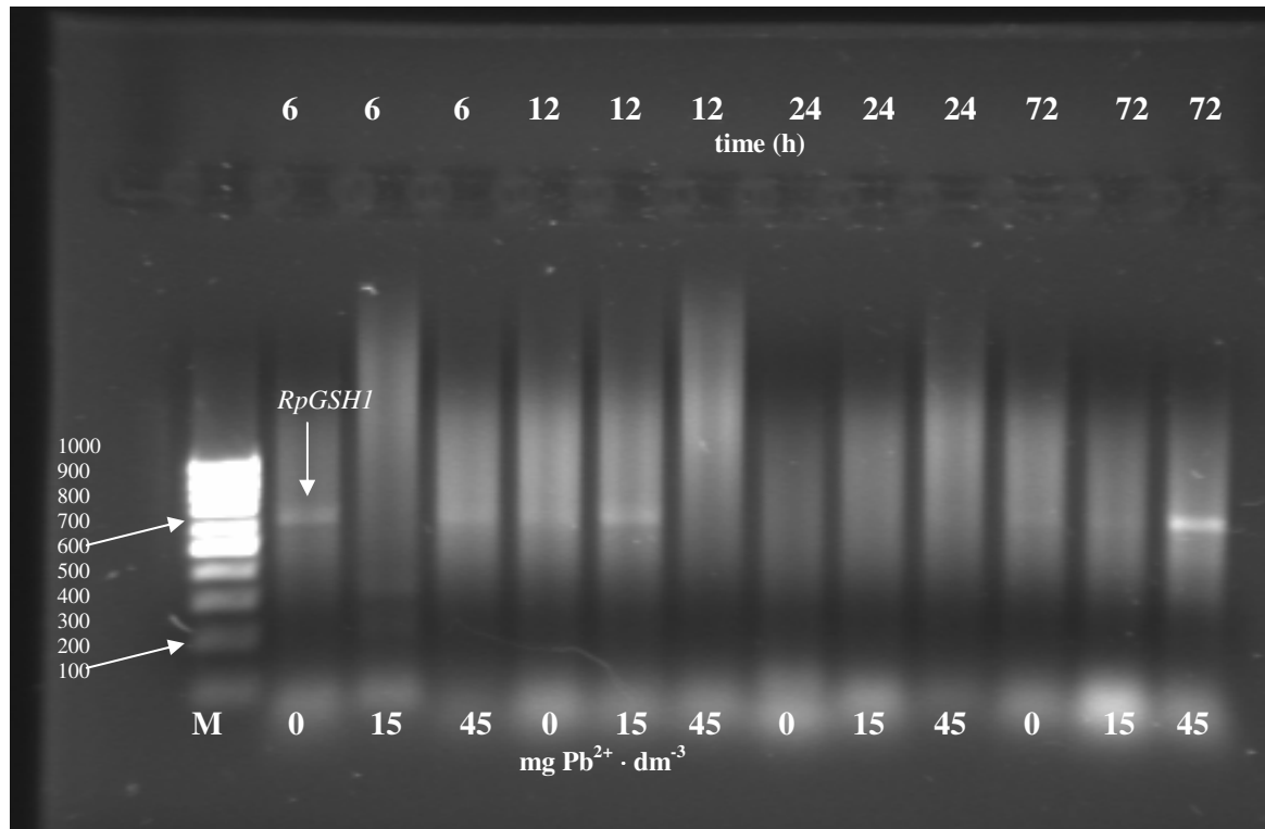
Phot. 1. The electropherogram of the amplified fragments of cDNA of genes encoding \gamma -glutamylcysteine synthetase (primers Gsh1F and Gsh1R) in Robinia pseudoaccacia roots, M – 100 bp DNA Ladder
