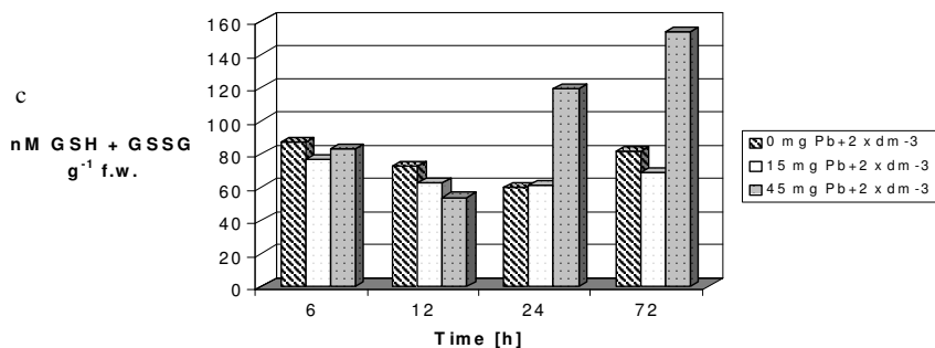
Fig. 1. Content of GSH+GSSG in organs (a – roots, b – stems, c – leaves) of Robinia pseudoacacia after 6, 12, 24, 72 hours of treatment with different dose of lead
