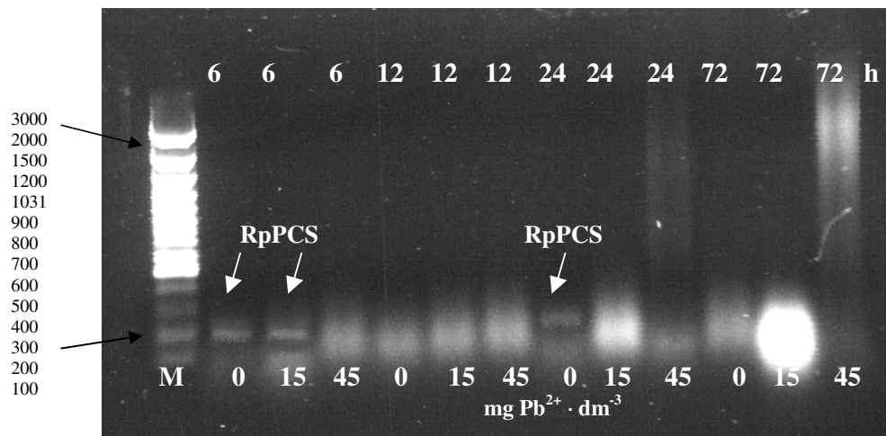
Phot. 2. The electrophorogram of the amplified fragments of cDNA of genes encoding of \gamma -phytochelatin synthase (primers AtPCS 5 and AtPCS 6) in Robinia pseudoaccacia roots, M – 100 bp DNA Ladder
